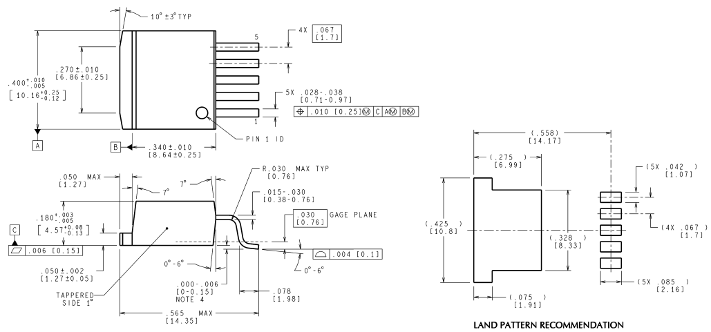
TO263 5-Lead, Molded, Surface Mount Package (TO263-5) NS Package Number TS5B For Order Numbers, refer to the "Ordering Information" section of this document.
